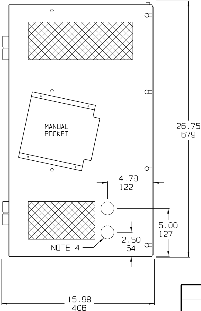
SIDE VIEW
