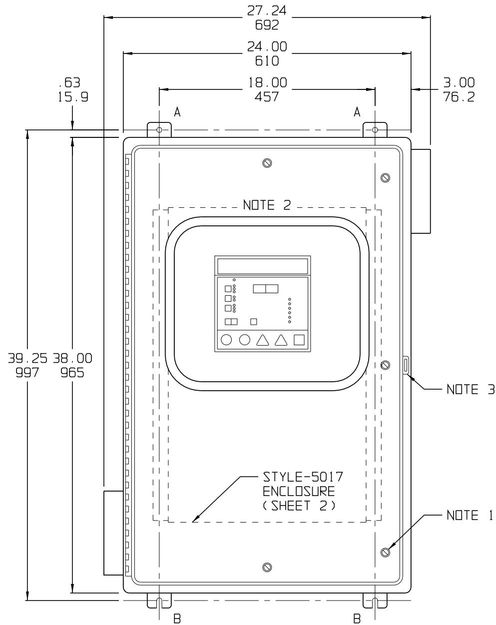
FRONT VIEW
