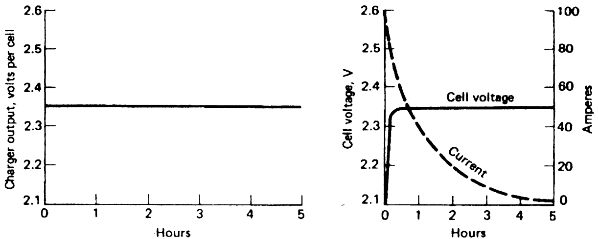
Fig. 1 - Representation of Constant Potential Charging
